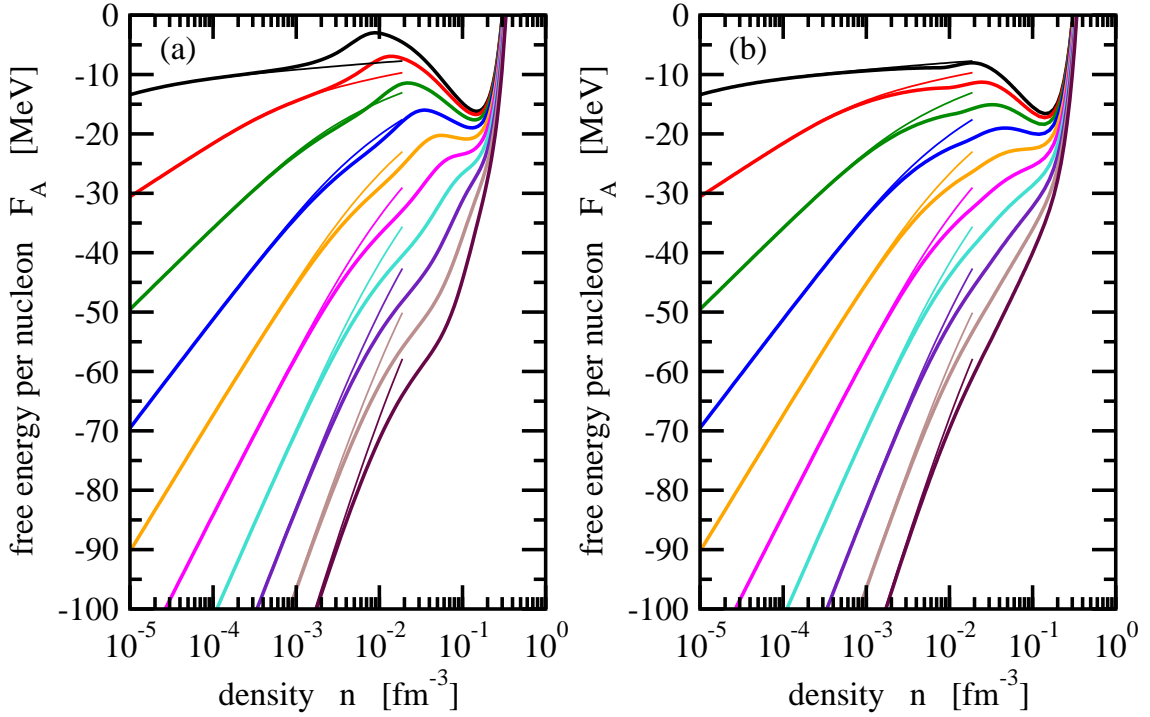
FIG. 7: (Color online) Free energy per nucleon F_A of symmetric nuclear matter as a function of the total density n for various temperatures T in the generalized RMF model (a) and the QS approach (b) with light clusters (thick solid lines). The result of the NSE calculation with light clusters is denoted by thin solid lines for low densities. See Fig. 2 for the color code.
