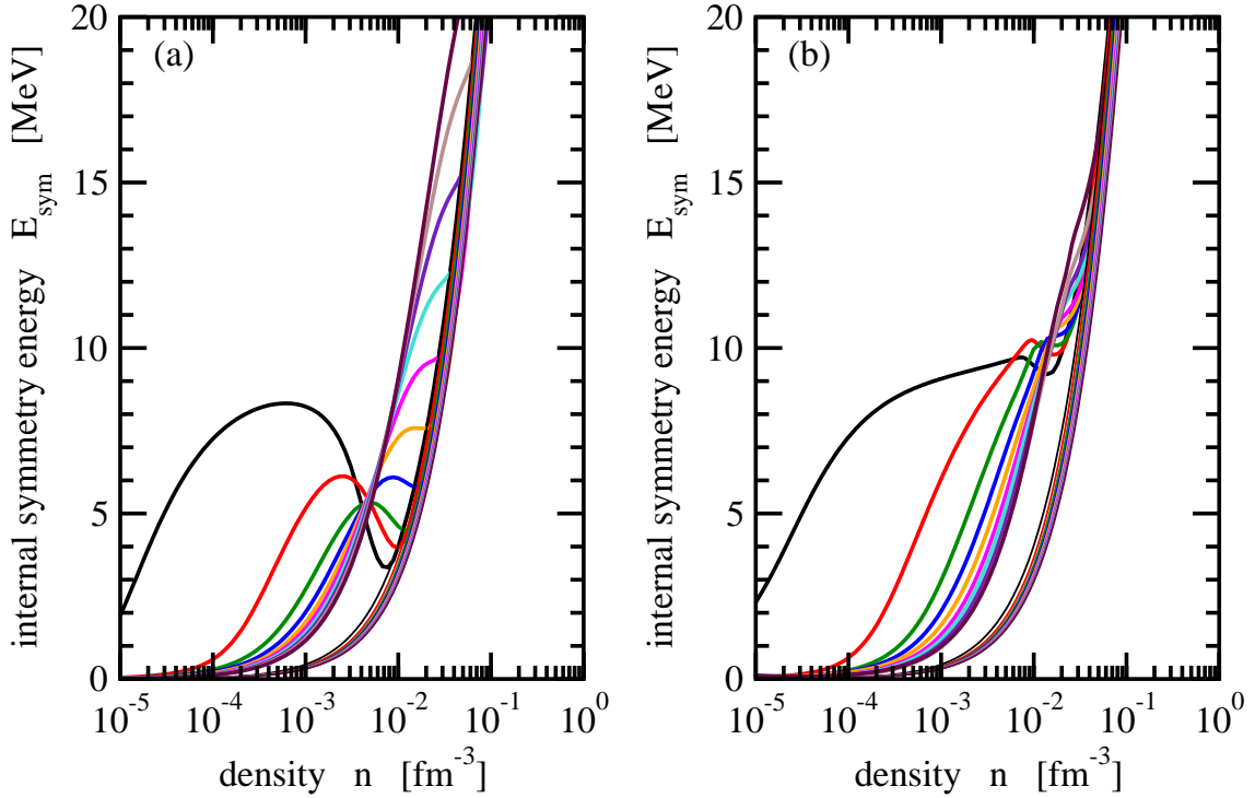
FIG. 13: (Color online) Internal symmetry energy E_{\text{sym}} as a function of the total density n for various temperatures T in the generalized RMF model (a) and the QS approach (b) with light clusters (thick solid lines). The result of the RMF calculation without clusters is denoted by thin solid lines for low densities. See Fig 2 for the color code.
