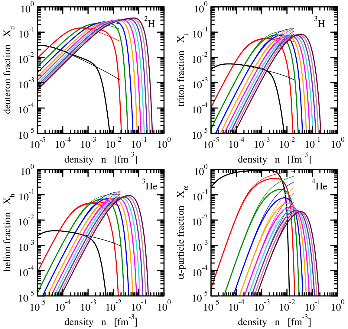
FIG. 3: (Color online) Cluster fractions X_i in symmetric nuclear matter as a function of the total density n for various temperatures T in the generalized RMF model (thick solid lines). The result of the NSE calculation with light clusters is denoted by thin solid lines for low densities. See Fig. 2 for the color code.
