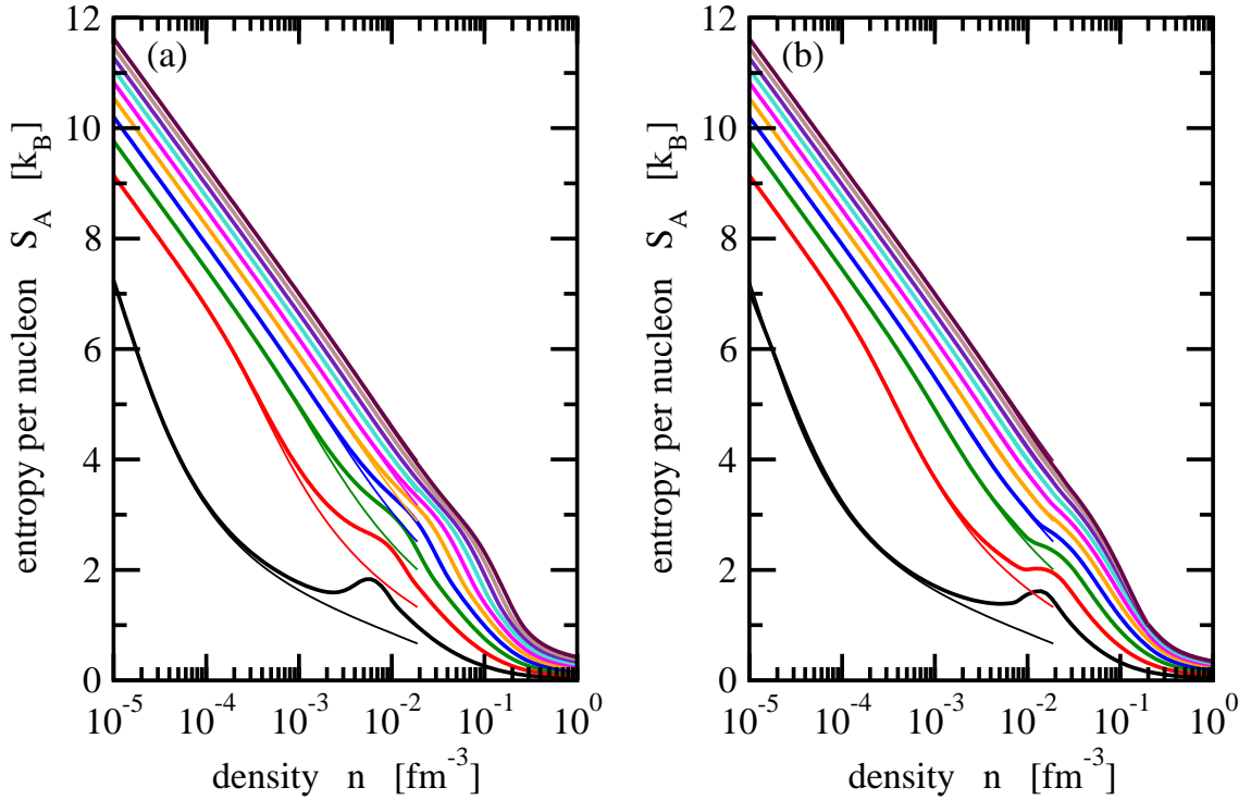
FIG. 9: (Color online) Entropy per nucleon S_A of symmetric nuclear matter as a function of the total density n for various temperatures T in the generalized RMF model (a) and the QS approach (b) with light clusters (thick solid lines). The result of the NSE calculation with light clusters is denoted by thin solid lines for low densities. See Fig. 2 for the color code.
