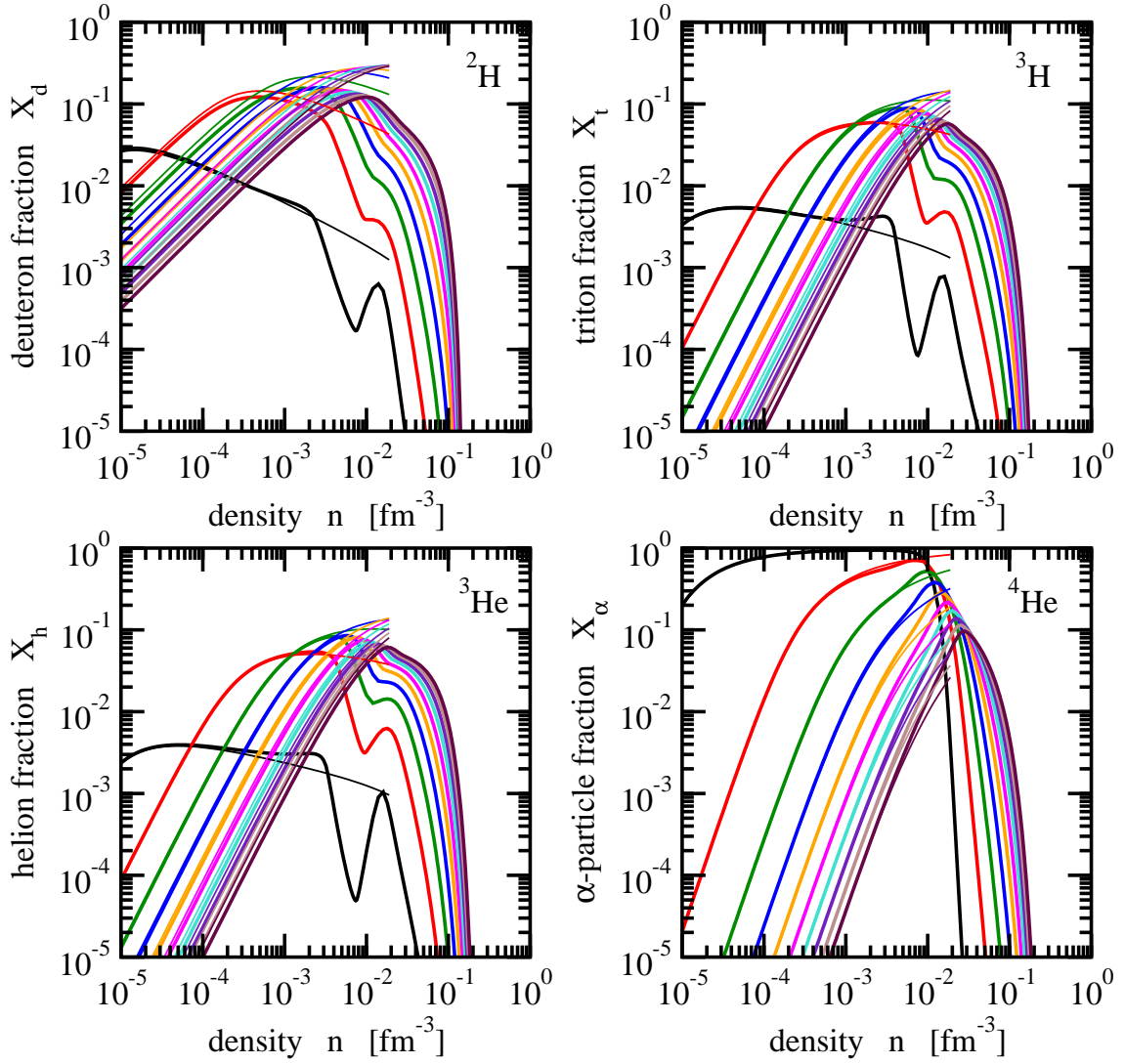
FIG. 4: (Color online) Cluster fractions X_i in symmetric nuclear matter as a function of the total density n for various temperatures T in the quantum statistical approach (thick solid lines). The result of the NSE calculation with light clusters is denoted by thin solid lines for low densities. See Fig. 2 for the color code.
