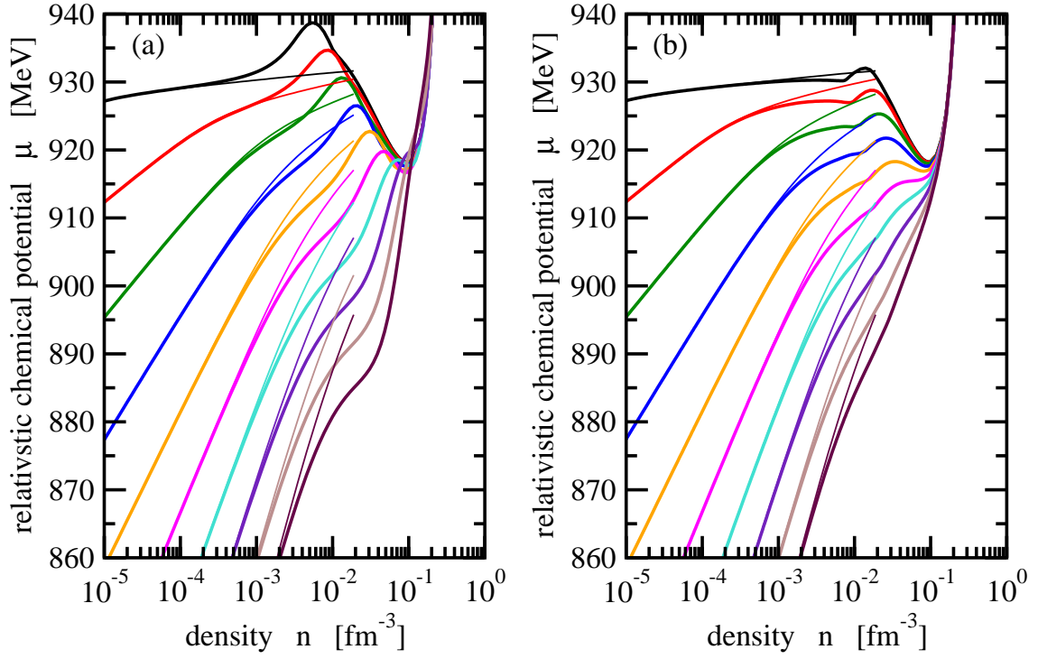
FIG. 6: (Color online) Relativistic baryon chemical potential \mu = (\mu_p + \mu_n)/2 of symmetric nuclear matter as a function of the total density n for various temperatures T in the generalized RMF model (a) and the QS approach (b) with light clusters (thick solid lines). The result of the NSE calculation with light clusters is denoted by thin solid lines for low densities. See Fig. 2 for the color code.
