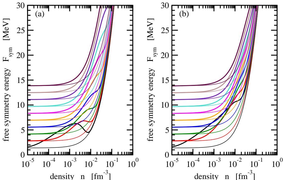
FIG. 14: (Color online) Free symmetry energy F_{\text{sym}} as a function of the total density n for various temperatures T in the generalized RMF model (a) and the QS approach (b) with light clusters (thick solid lines). The result of the RMF calculation without clusters is denoted by thin solid lines for low densities. See Fig. 2 for the color code.
