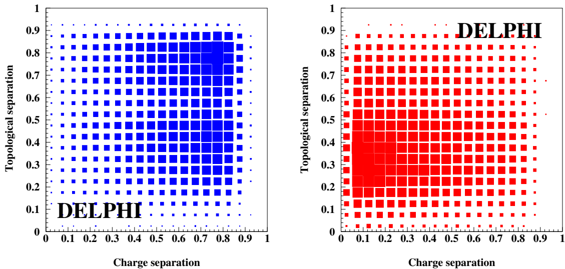
Fig. 10. Two-dimensional distribution of the topological and charge correlation variables for the signal B \rightarrow X_c \ell \bar{\nu}_\ell (left) and the main background B \rightarrow X_c \ell \nu (right)
