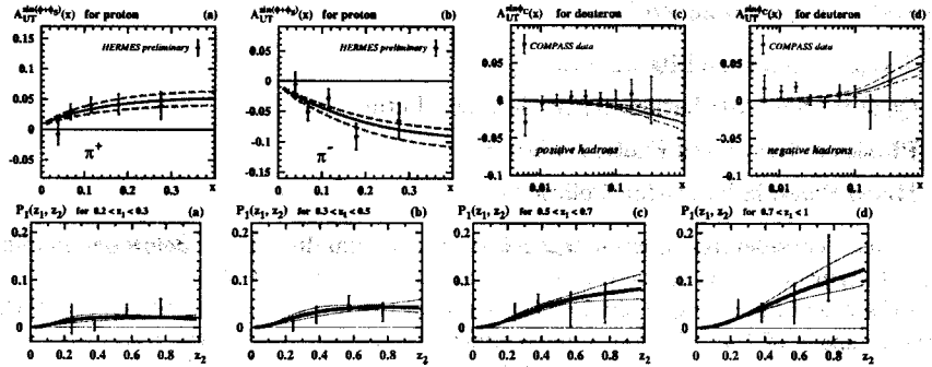
Fig. 1: Top: The HERMES (a,b) and COMPASS (c,d) data on Collins asymmetry. Bottom: The BELLE data on Collins effect.
