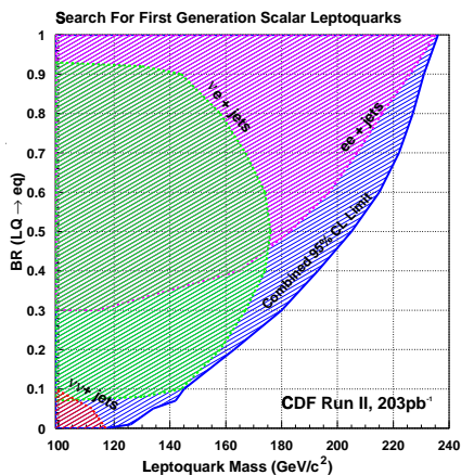
FIG. 1: LQ mass exclusion regions at 95% C.L. as a function of \text{Br}(\text{LQ} \rightarrow e q) .
