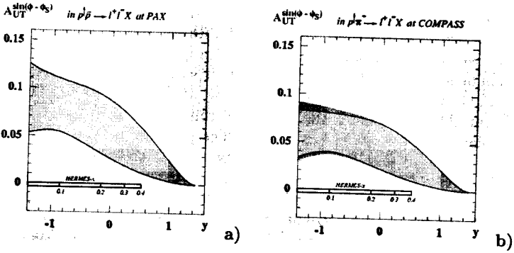
Fig. 1: Azimuthal asymmetries A_{UT}\sin(\phi_h - \phi_S) in production of the Drell-Yan lepton pair, p^\dagger h \rightarrow \mu^+\mu^- X , depending on rapidity y : (a) for kinematics of the PAX experiment, where hadron h = \bar{p} , (b) for kinematics of the COMPASS experiment, where h = \pi^- . The shaded area corresponds to 1\sigma uncertainty of the fit.
