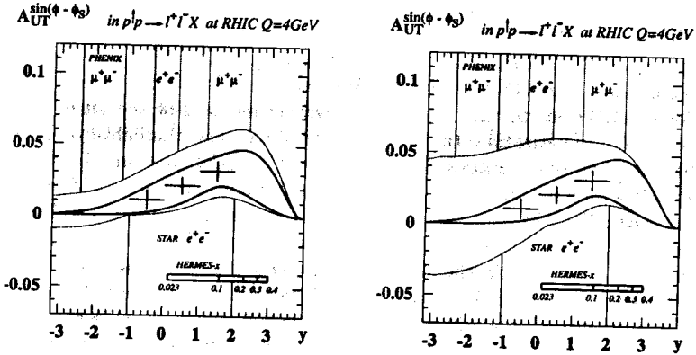
Fig. 2: The azimuthal SSA A_{UT}^{\sin(\phi - \phi_S)} in the Drell-Yan lepton pair production, p^\dagger p \rightarrow l^+l^- X , as a function of y for the kinematics of the RHIC experiment with \sqrt{s} = 200 GeV. The left and right plots correspond to different ansatze for Siverts antiquark distributions. For Q = 4 GeV we show the estimated statistical error for STAR.
