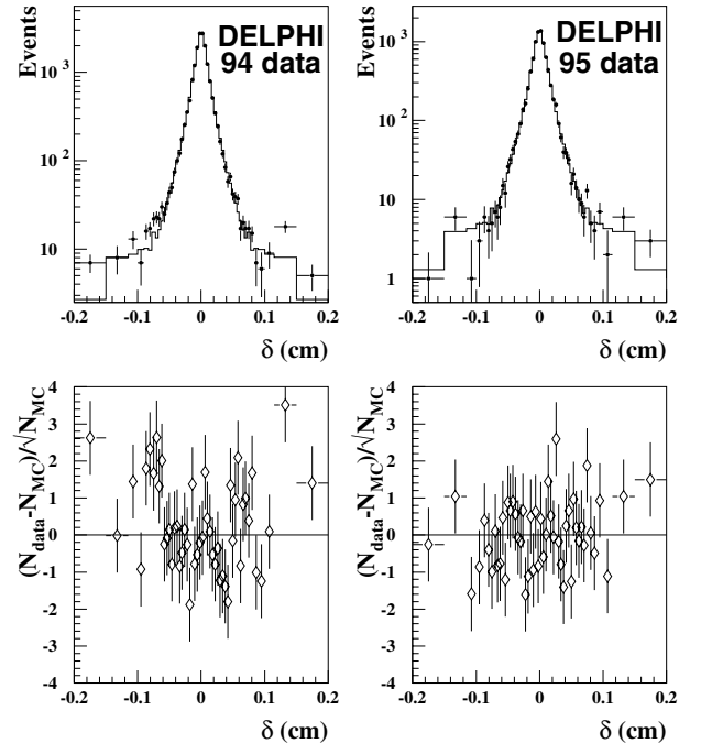
Fig. 6. Distributions of the miss distance for the 1994 and 1995 data samples, points with error bars are data, the histogram the fitted distribution. The lower plots show the pulls of the differences between the observed data and the expected events from the simulation
