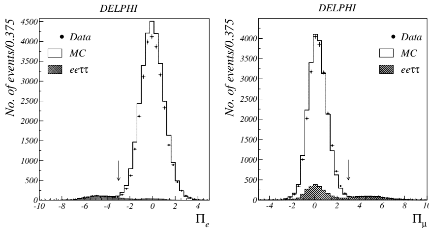
Fig. 3. Distribution of the dE/dx pull for the electron hypothesis (left) and for the muon hypothesis (right) with all selection cuts applied except the cut on the variable shown. Points are 1999 data, the open histogram is the background, and the shaded histogram shows the e^+e^- \rightarrow e^+e^-\tau^+\tau^- signal events. The simulation is not corrected for the trigger efficiency
