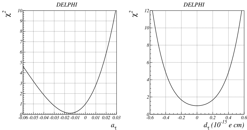
Fig. 8. \chi^2 as a function of anomalous magnetic moment and as a function of electric dipole moment
