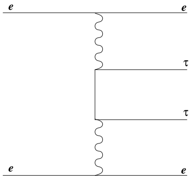
Fig. 1. The dominant diagram for the reaction e^+e^- \rightarrow e^+e^-\tau^+\tau^-
