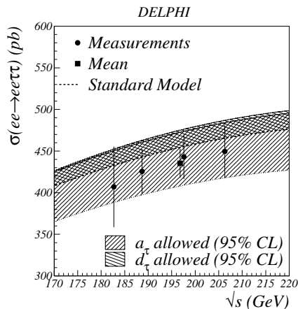
Fig. 9. Measured cross-section (circles), average LEP2 cross-section (square) and SM expectation as a function of \sqrt{s} . The two bands show the cross-section variation allowed due to anomalous magnetic and electric dipole moments within 95% limits from this analysis
