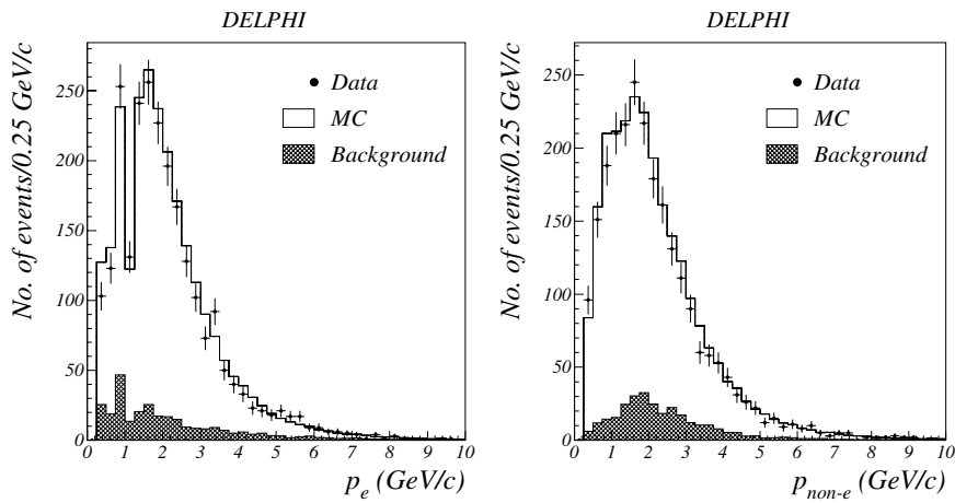
Fig. 5. Momentum distribution for electron candidates (left) and non-electron candidates (right) for selected events from 1997–2000 data. The distributions of simulated events are corrected for trigger efficiency. The dip in the electron momentum distribution near 1 GeV/c is caused by the cut against protons: the electron and proton dE/dx are equal in this region of momentum
