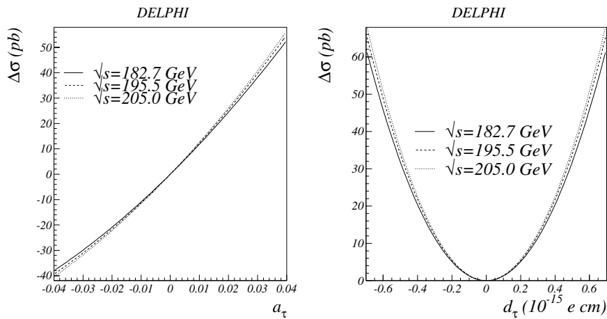
Fig. 7. Total cross-section change as a function of anomalous magnetic moment and as a function of electric dipole moment
