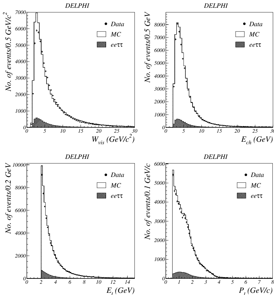
Fig. 2. The distributions of invariant mass, total energy, transverse energy and transverse momentum of the pair of charged particles. Preselection cuts are applied. The points are 1999 data, the open histogram is the simulation of background processes and the shaded histogram is the simulation of e^+e^- \rightarrow e^+e^-\tau^+\tau^- events. The simulation is not corrected for the trigger efficiency
