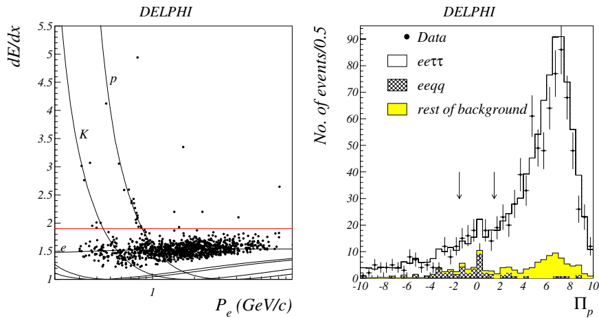
Fig. 4. Left: specific energy loss as a function of particle momentum for electron candidates after preselection cuts and the cuts on the electron and muon pulls. The horizontal line shows the first cut against kaons and protons. The points are 1999 data. Right: distribution of dE/dx pull for proton hypothesis for electron candidates. The hatched histogram is the background from e^+e^- \rightarrow e^+e^-q\bar{q} events and the shaded histogram is the rest of the background. The cuts against protons are indicated by arrows. All other selection cuts are applied. The points are 1999 data
