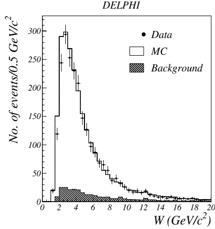
Fig. 6. Visible invariant mass distribution for selected events for combined 1997–2000 data. The distribution of simulated events is corrected for trigger efficiency. The mass was calculated using all detected charged particles and photons. The simulation was corrected for the trigger efficiency
