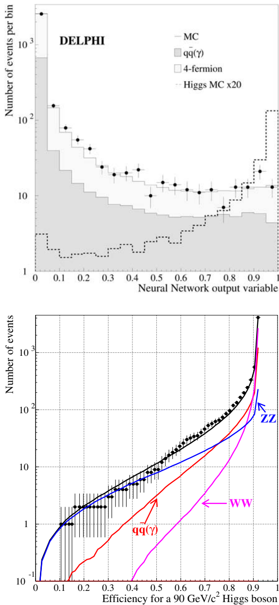
Fig. 19. hA hadronic channel: Top: distributions of the ANN variable for the expected SM background processes (full histograms), the data from the years 1999 and 2000 (dots) and the expected m_A = m_h = 90 \text{ GeV}/c^2 Higgs signal (dashed histogram, normalised to 20 times the expected rate). Bottom: curve of the expected SM background rate for all data from 1999 and 2000 as a function of the efficiency for the same signal when varying the cut on the ANN variable. The different background contributions are shown separately. The dots show the data
