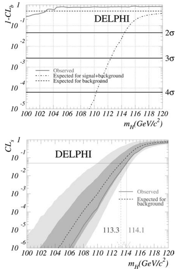
Fig. 25. SM Higgs boson: confidence levels as a function of m_H . Top: 1 - \text{CL}_b for the background hypothesis. The full curve is the observation, the dashed curve is the median expected for background only, and the dash-dotted curve is the median expected at a particular m_H value when tested for that m_H value. A signal would appear as a downward deviation. Bottom: \text{CL}_s , the pseudo-confidence level for the signal hypothesis. Curves are the observed (full) and expected median (dashed) confidences from experiments with only background channels while the bands correspond to the 68.3% and 95.0% confidence intervals for the hypothesis of only background processes. The intersections of the curves with the horizontal line at 5% define the expected and observed 95% CL lower limits on m_H
