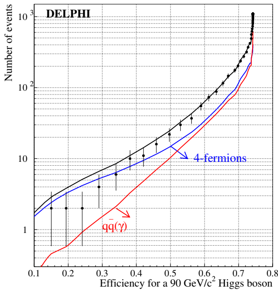
Fig. 11. H\nu\bar{\nu} channel, low mass analysis: the observed rate and that expected from the SM background processes as a function of the efficiency for a 90 \text{ GeV}/c^2 Higgs signal when varying the cut on the likelihood variable. The total background and different background contributions are shown separately. The dots represent the data
