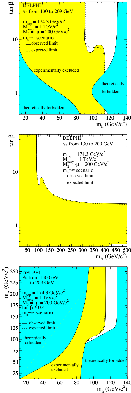
Fig. 28. MSSM Higgs bosons: regions excluded at 95% CL by the searches in the combined hZ and hA channels, in the m_h^{\max} scenario. The dark shaded areas are the regions not allowed by the MSSM model in this scenario. The dashed curves show the median expected limits
