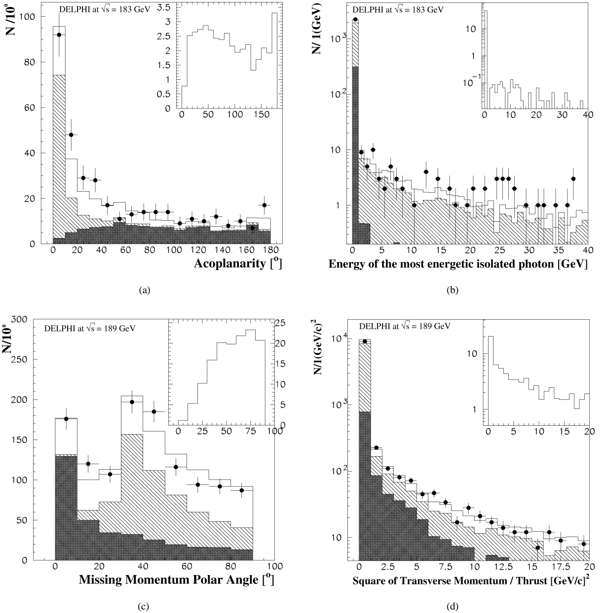
Fig. 3. Distribution of (a) acoplanarity, (b) energy of the most energetic isolated photon, (c) angle between the missing momentum and the beam-axis and (d) square of transverse momentum with respect to the thrust axis divided by the thrust, requiring that the events had two clusters of well reconstructed neutral and charged particles, less than 7 charged particles and a total transverse momentum above 4 \text{ GeV}/c . For the acoplanarity and the missing momentum polar angle distributions it was also required that the square of the transverse momentum with respect to the thrust axis divided by the thrust was above 0.75 (\text{GeV}/c)^2 and above 1 (\text{GeV}/c)^2 , respectively. The points with error bars show the real data, while the white histograms show the total simulated background. The distributions corresponding to the \gamma\gamma background and the Bhabha scattering are shown as dark and hatched histograms, respectively. An example of the two-body decay mode \tilde{\chi}^\pm \rightarrow \tau^\pm + J behaviour for \tan\beta = 2 , \mu = 100 \text{ GeV}/c^2 and M_2 = 400 \text{ GeV}/c^2 is shown in the inserts for each plot.
