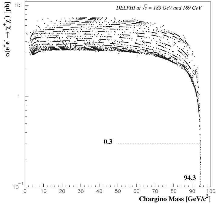
Fig. 5. Expected e^+e^- \rightarrow \tilde{\chi}^+\tilde{\chi}^- cross-section at 189 GeV (dots) as a function of the chargino mass, assuming a heavy sneutrino ( M_{\tilde{\nu}} \geq 300 \text{ GeV}/c^2 ). The dots correspond to the generated events at different chargino masses for the MSSM parameter ranges: 40 \text{ GeV}/c^2 \leq M_2 \leq 400 \text{ GeV}/c^2 , -200 \text{ GeV}/c^2 \leq \mu \leq 200 \text{ GeV}/c^2 and 2 \leq \tan \beta \leq 40 . At the 95% confidence level, assuming the chargino decays mainly to \tau^{\pm}J , the maximum allowed chargino-production cross section in the excluded mass region is 0.3 pb and the corresponding lower mass limit is 94.3 \text{ GeV}/c^2 .
