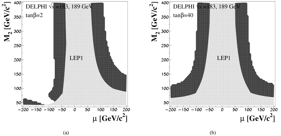
Fig. 6. Regions in the \mu , M_2 parameter space excluded at the 95% confidence level for (a) \tan \beta = 2 and (b) \tan \beta = 40 , assuming M_{\tilde{\nu}} \geq 300 \text{ GeV}/c^2 . The exclusion area obtained with the \tilde{\chi}^{\pm} \rightarrow \tau^{\pm}J search is shown in dark grey and the corresponding area excluded by the LEP1 data [23] is shown in light grey. The hole seen on plot (a) around M_2 = 50 \text{ GeV}/c^2 and \mu = -120 \text{ GeV}/c^2 is due to the low branching ratio (below 5%) for the \tilde{\chi}^{\pm} \rightarrow \tau^{\pm}J .
