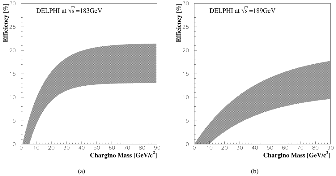
Fig. 4. Chargino detection efficiency as a function of the chargino mass for (a) \sqrt{s} = 183 GeV and (b) \sqrt{s} = 189 GeV, considering only the two-body decay mode \tilde{\chi}^{\pm} \rightarrow \tau^{\pm} + J . The bands correspond to the statistical uncertainties combined with the effect of generating events with different MSSM parameters M_2 and \mu , which have been varied in the ranges 40 \text{ GeV}/c^2 \leq M_2 \leq 400 \text{ GeV}/c^2 and -200 \text{ GeV}/c^2 \leq \mu \leq 200 \text{ GeV}/c^2 , for \tan \beta = 2 .
