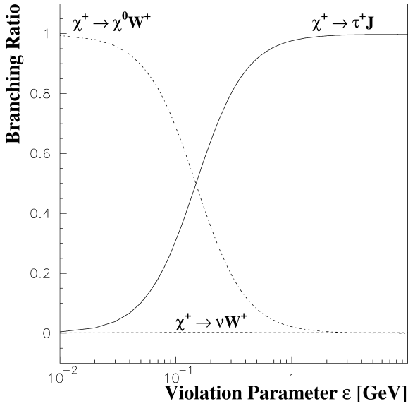
Fig. 1. Chargino decay branching ratios as a function of the effective R -parity-violation parameter \epsilon for \tan\beta = 2 , \mu = 100 \text{ GeV}/c^2 and M_2 = 400 \text{ GeV}/c^2 .
