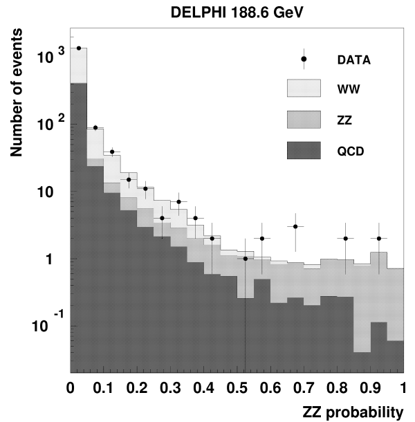
Fig. 2. Distribution of the ZZ probability for all events at 188.6 GeV in the four-jet channel.
