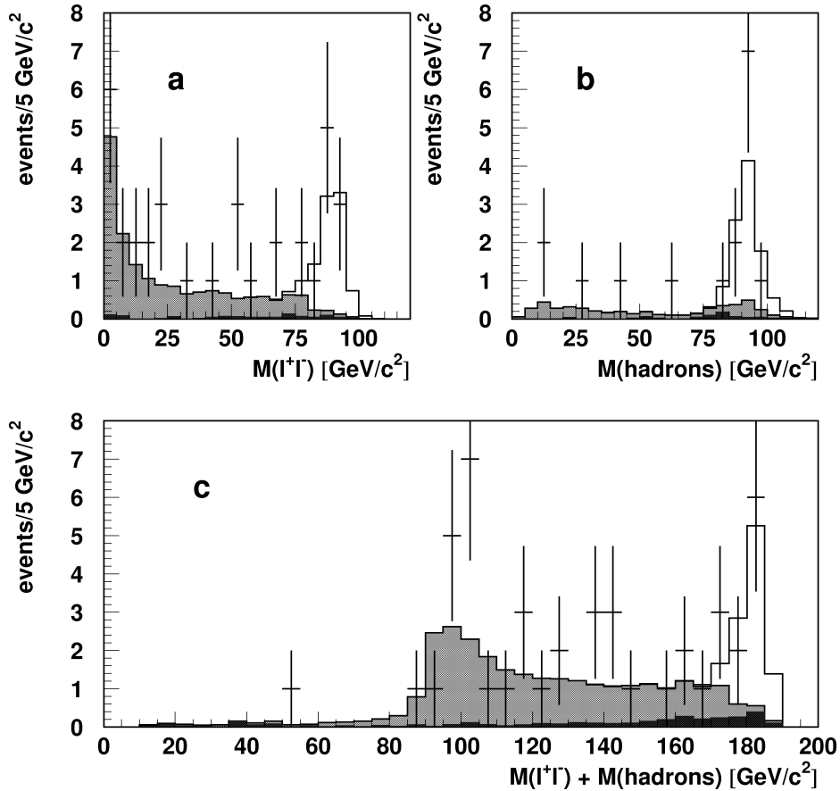
Fig. 3. (a) the distribution of the mass of the l^+l^- pair when the mass of the hadron system is within 15 \text{ GeV}/c^2 of the nominal Z mass; (b) the distribution of the mass of the hadron system when the mass of the l^+l^- pair is within 15 \text{ GeV}/c^2 of the nominal Z mass; (c) the distribution of the sum of the masses of the l^+l^- pair and of the hadron system. The points are the data taken at 182.6 \text{ GeV} and at 188.6 \text{ GeV} , and the histogram is the simulation prediction. The contribution from the signal, as defined in Section 3, is indicated by the empty histogram. The contributions from backgrounds are indicated with light grey when arising from from l^+l^-q\bar{q} final states, and with dark filling otherwise.
