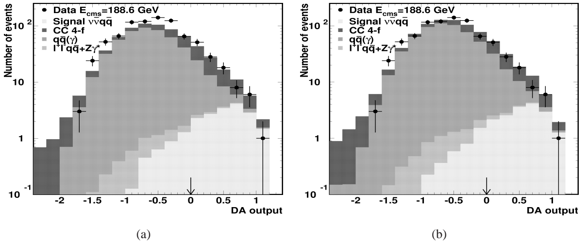
Fig. 4. \nu\bar{\nu}q\bar{q} channel: the second-order discriminant for the data at 188.6 GeV, for the expected signal (light) and for the backgrounds from l^+l^-q\bar{q} and Z\gamma^* (light grey), q\bar{q}(\gamma) (dark grey) and W\bar{e}e and WW (dark, CC 4f in the legend) processes are shown, using the nominal (a) and corrected (b) simulation, following the procedure described in the text. The main effect from the correction procedure was to increase the q\bar{q}(\gamma) background component. The arrow indicates the cut used to remove the part of the distribution where the q\bar{q}(\gamma) background dominates, in order to reduce the systematic error as described in the text.
