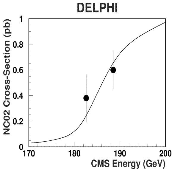
Fig. 5. Combined NC02 cross-sections measured from data collected in 1997 and 1998. The solid curve was computed using the YFSZZ Monte Carlo [24]. Values obtained with the EXCALIBUR Monte Carlo were within \pm 1\% of those obtained with YFSZZ.
