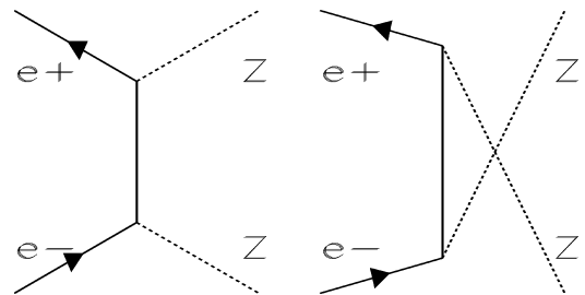
Fig. 1. The Feynman graphs for on-shell ZZ production (referred to as the NC02 graphs).
