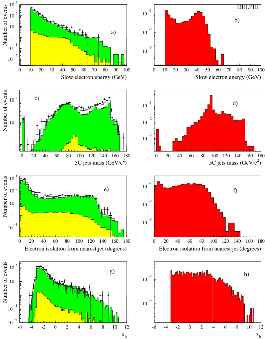
Fig. 2a–h. He^+e^- channel: distributions of some analysis variables as described in the text, at the preselection level. The plots on the left-hand side show a comparison between 188.7 GeV data (dots) and simulated background events (solid line) normalised to the experimental luminosity. The dark grey areas represent the contribution of the q\bar{q}(\gamma) background and the light grey area the e^+e^-q\bar{q} contribution. The expected normalised distributions of the same variables for a signal at 95 \text{ GeV}/c^2 are represented on the right-hand side. Note the different y-scales
