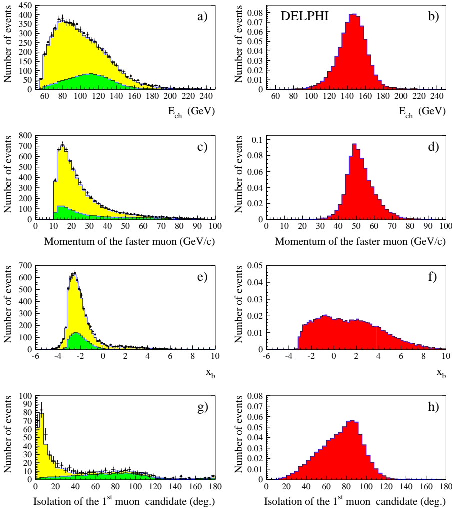
Fig. 4a–h. H\mu^+\mu^- channel: distributions of some analysis variables as described in the text, at the preselection level (a to f) or after the lepton pair selection (g and h). The dark grey area represents the contribution of the q\bar{q}(\gamma) background and the light grey area the 4 fermions contribution. The expected normalised distribution for the signal (with m_H = 95 \text{GeV}/c^2 ) is represented on the right-hand column
