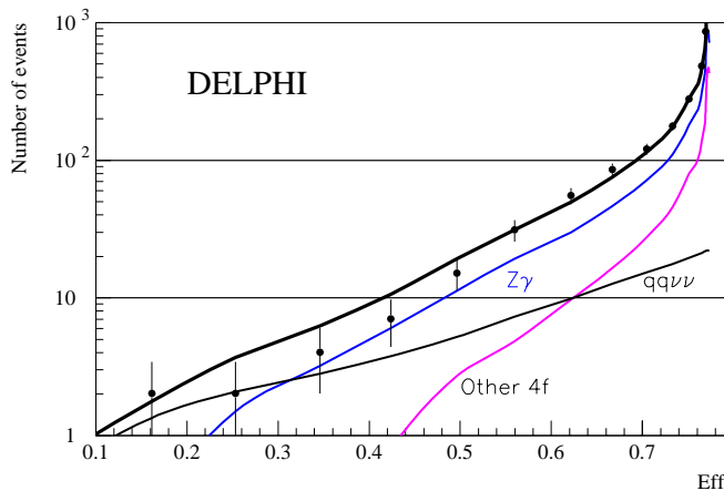
Fig. 8. H\nu\bar{\nu} channel: Efficiency versus total background as a result of varying the cut on the Likelihood. The contribution of different backgrounds are shown separately. Points with error bars are the data, and the thick black line shows the total expected background
