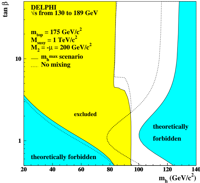
Fig. 18. Regions in the (m_h, \tan\beta) plane excluded at 95% CL by the searches in the hZ and hA channels up to \sqrt{s} = 189 GeV. Two extreme hypotheses for the mixing in the stop sector are considered. The regions not allowed by the MSSM model for m_{\text{top}} = 175 GeV/ c^2 , M_{\text{SUSY}} = 1 TeV/ c^2 , M_2 = -\mu = 200 GeV/ c^2 and m_A < 1 MeV/ c^2 or m_A > 1 TeV/ c^2 are also indicated (shaded for the m_h^{\text{max}} scenario)
