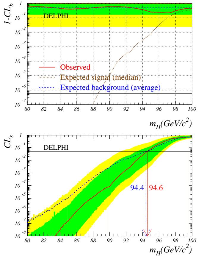
Fig. 15. Confidence levels as a function of the SM Higgs boson mass. Curves are shown for the expected (dashed) and observed (solid) confidences and the bands correspond to the 68.3% and 95% confidence intervals. Top: Confidence level in the background hypothesis. Bottom: Confidence level in the signal hypothesis. The intersections of the horizontal line at 5% with the curves define the expected and observed 95% CL lower limits on the Higgs boson mass
