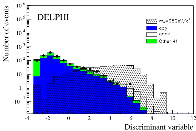
Fig. 7. H\nu\bar{\nu} channel: Distributions of the discriminant variable for the expected background events (full histograms), data (points) and a Higgs signal with m_H = 95 \text{GeV}/c^2 (dashed histogram) are shown. The normalisation for the Higgs signal is 100 times the expectation
