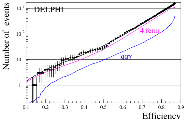
Fig. 11. Hq\bar{q} channel: Efficiency versus total background as a result of varying the cut on the Likelihood. The contribution of different backgrounds are shown separately. Points with error bars are the data and the upmost black line the total expected background
