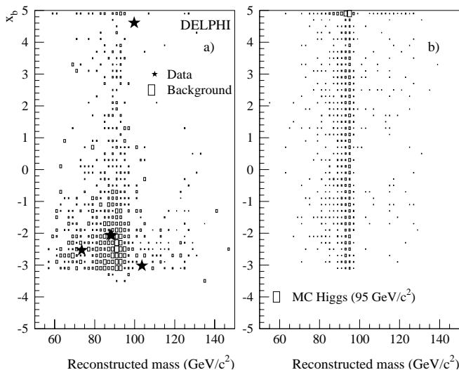
Fig. 3a,b. He^+e^- channel: distributions of the global b-tagging variable versus the fitted recoil mass for data, background and simulated signal events with m_H = 95 GeV/c^2 at 188.7 GeV. These distributions are the inputs for the Confidence Levels computation
