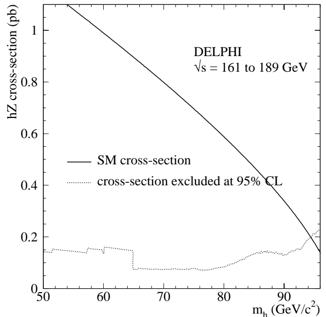
Fig. 17. 95% CL excluded cross-sections as a function of the Higgs boson mass compared with the SM expectation
