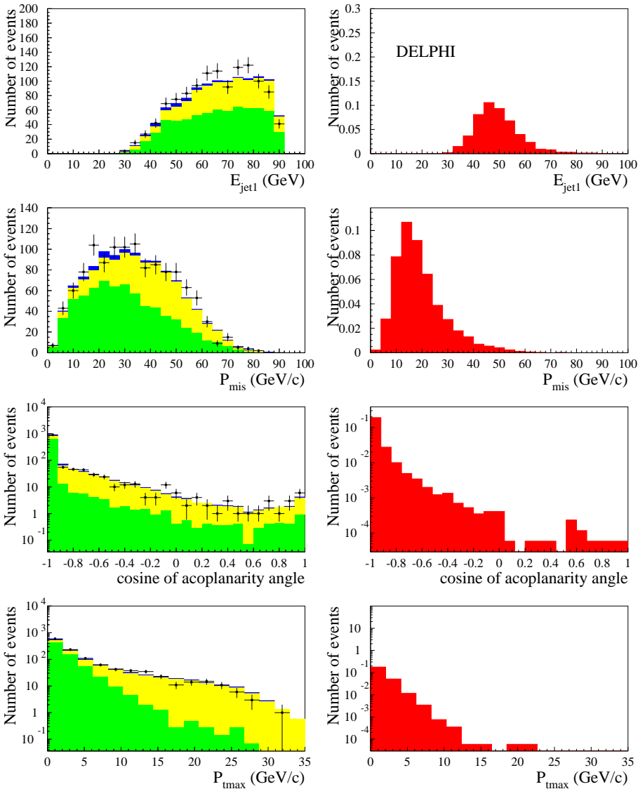
Fig. 6a–h. H\nu\bar{\nu} channel: distributions of the main analysis variables as described in the text, at the preselection level. The points with error bars represent the data. The left hand side histograms show the different backgrounds and the right hand side histograms show the signal distributions for m_H = 95 \text{ GeV}/c^2
