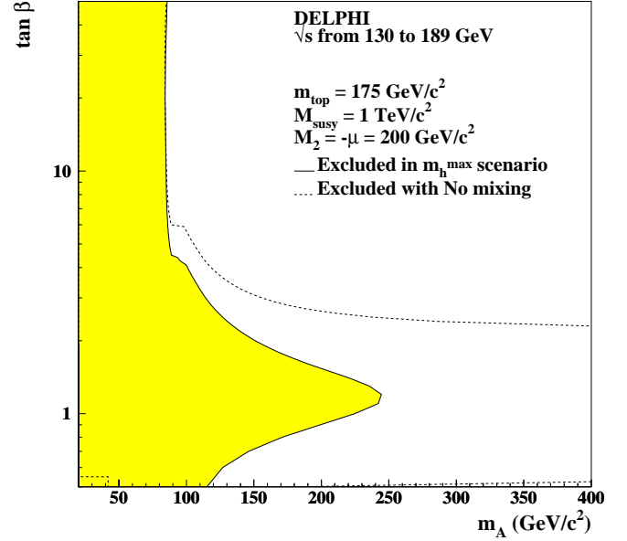
Fig. 19. Regions in the (m_A, \tan\beta) plane excluded at 95% CL by the searches in the hZ and hA channels up to \sqrt{s} = 189 GeV. Two extreme hypotheses for the mixing in the stop sector are presented
