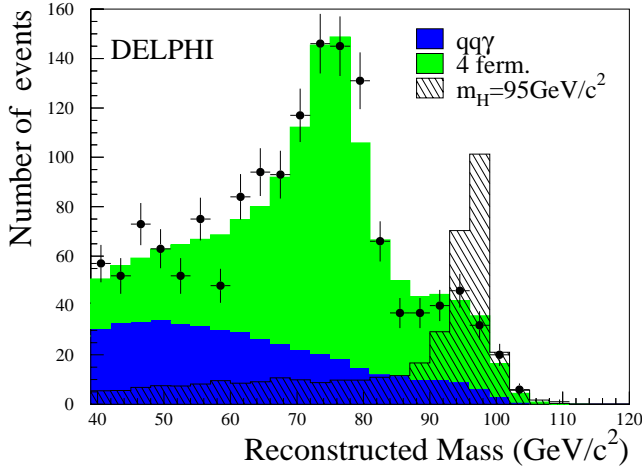
Fig. 10. Hq\bar{q} channel: The reconstructed mass at the preselection level. Note that the signal corresponds to 400 times the luminosity for clarity
