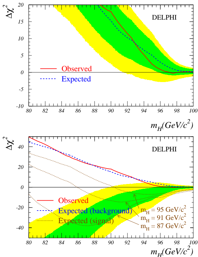
Fig. 16. The effective \Delta\chi^2 with which each SM Higgs mass is excluded (solid) and the expected value of the same (dashed). Top: Expectation in case of background only; the dark/light bands correspond to the 68.3% / 95% confidence intervals. Bottom: the bands represent the confidence intervals for the minima of the expectation curves in case of a signal (dotted lines)
