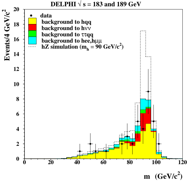
Fig. 14. Final distribution of the reconstructed Higgs boson mass when combining all hZ analyses at 182.7 and 188.7 GeV. Data are compared with background expectations. The expected spectrum, with the correct rate, from a signal at 90 \text{ GeV}/c^2 is also shown added to the background contributions, as the dotted histogram
