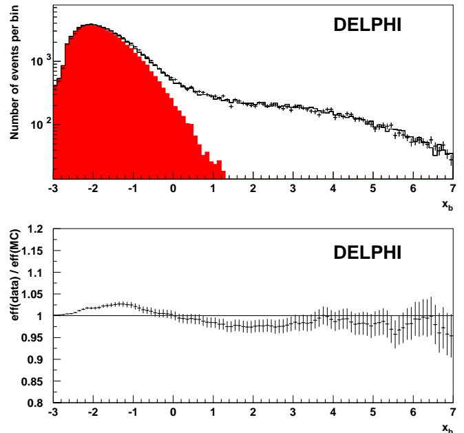
Fig. 1. Distributions of the combined b-tagging variable x_b , in data (points) and simulation (histogram). The contribution of udsc-quarks is shown as the dark histogram. Bottom: the ratio of the tagging rates in the data and the simulation as a function of the cut in the b-tagging variable
