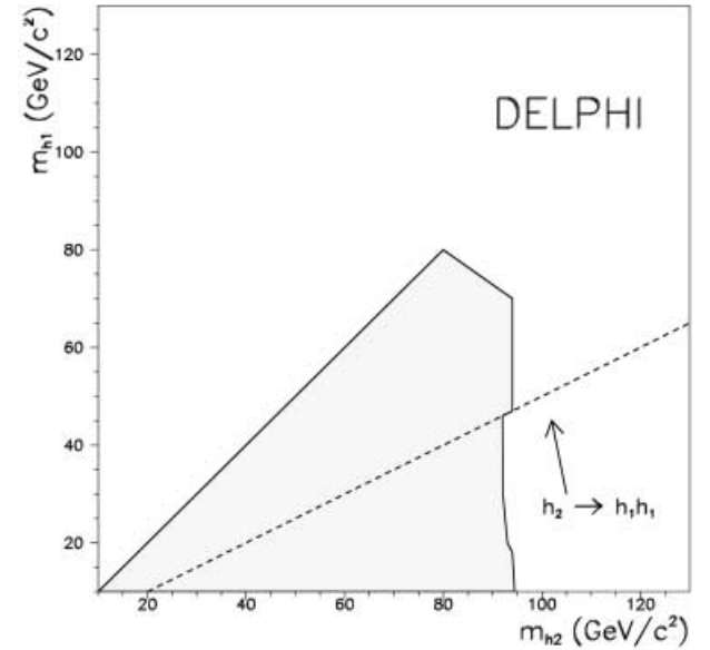
Fig. 21. Excluded regions at the 95% CL a) in the CP-conserving model (with dominant b -decays (ZONE I) and dominant non- b decays (ZONE II)) and b) in the CP-violating model
