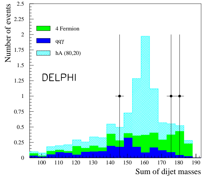
Fig. 13. hA hadronic channel: Mass distribution for the sum of the di-jets in data and MC at the end of the hA 4-jet analysis at the 55% efficiency level. The signal, with m_A = 80 \text{ GeV}/c^2 and \tan\beta = 20 is normalised to the data
