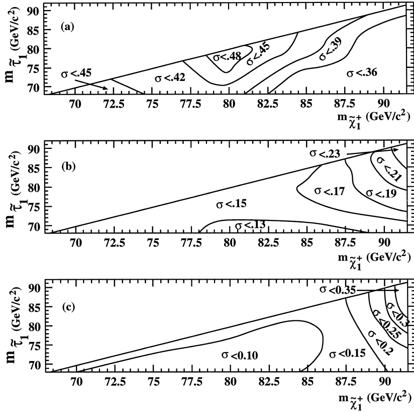
Fig. 3. Limits in pb on lightest chargino pair production cross-section at 95% CL. Limits are shown as functions of m_{\tilde{\chi}_1^+} and m_{\tilde{\tau}_1} for (a) m_{\tilde{G}} = 1 \text{ eV}/c^2 , (b) m_{\tilde{G}} = 100 \text{ eV}/c^2 and (c) m_{\tilde{G}} = 1000 \text{ eV}/c^2 .
