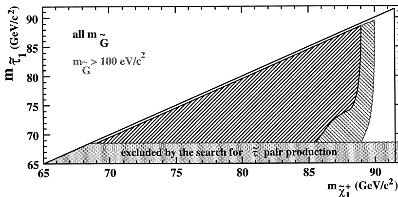
Fig. 4. Areas excluded at 95% CL in the (m_{\tilde{\chi}_1^+}, m_{\tilde{\tau}_1}) plane. The positive-slope area is excluded for all m_{\tilde{G}} . The negative-slope area is excluded for m_{\tilde{G}} \geq 100 \text{ eV}/c^2 . The grey area is excluded by the direct search for stau pair production.
