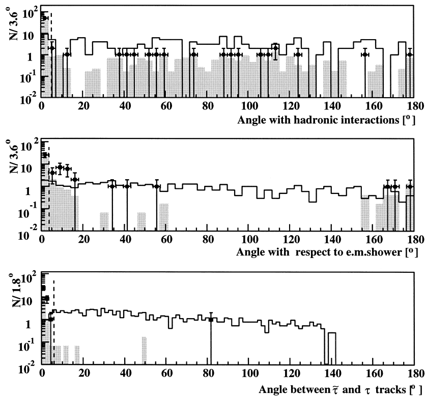
Fig. 2. Angle between the hadronic interaction (if any) and the reconstructed vertex (above), angle between the electromagnetic shower and the direction defined by the difference between the momenta of \tilde{\tau}_1 and its associated \tau , defined at the crossing point (middle), and angle between the tracks of the kink (below), for real data (dots), expected Standard Model background (dark histogram) and simulated signal for m_{\tilde{\chi}_1^+} = 85 \text{ GeV}/c^2 and m_{\tilde{\tau}_1} = 69 \text{ GeV}/c^2 decaying with a mean distance of 50 cm (blank histogram). The segmented lines indicate selection criteria imposed as explained in Ref. [9].
