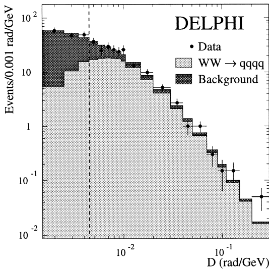
Fig. 1. Distribution of the D variable for 4-jet events. The points show the data and the histograms are the predicted distributions for signal and background. The latter includes small contributions from other WW channels.
