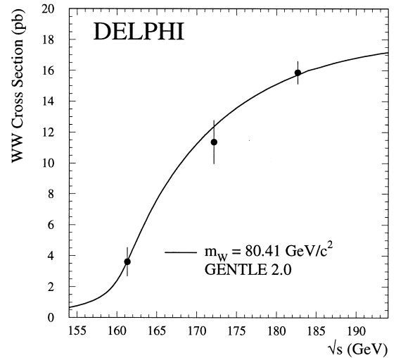
Fig. 3. Measurements of the W^+ W^- cross-section compared with the Standard Model prediction using m_W = 80.41 \text{ GeV}/c^2 [11].
