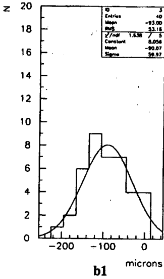
Fig.14. Deviations measured data from nominal dimensions for spacer 5.
