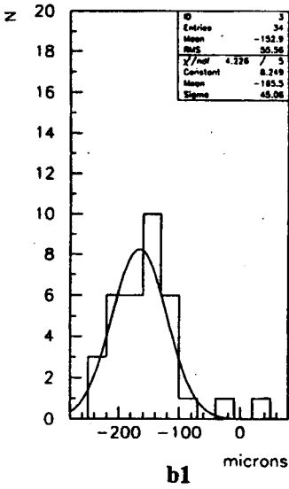
Fig.18. Deviations measured data from nominal dimensions for spacer 9.
