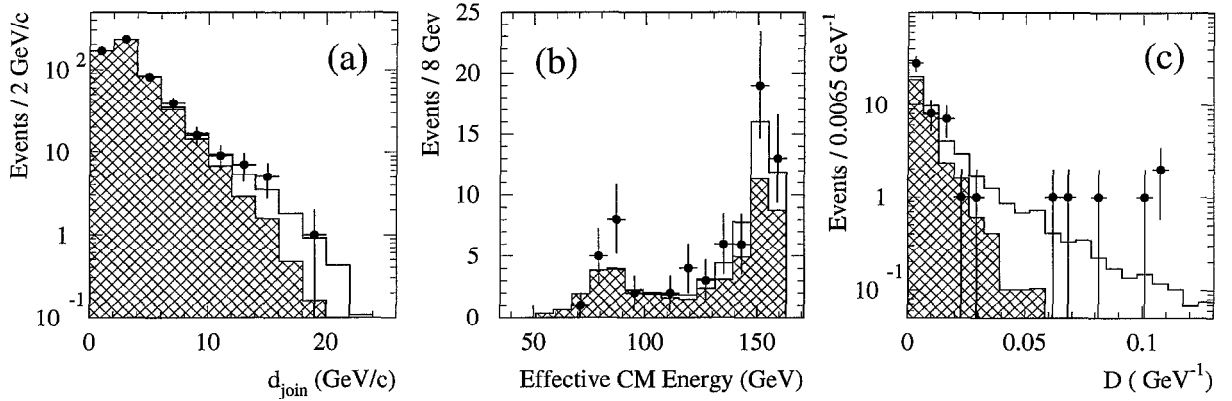
Fig. 1. Fully hadronic final state: comparison of data (points with error bars) with simulated q\bar{q}(\gamma) background (cross-hatched areas) and WW signal (white areas) normalised to the fitted cross-section. (a) Differential 3-jet rate (number of events changing from 4 to 3 jets) as function of d_{\text{join}} ; (b) effective centre-of-mass energy for events with at least 4 jets; (c) D variable (as defined in the text) for 4-jet events with effective centre-of-mass energy greater than 115 GeV.
