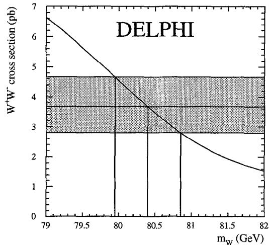
Fig. 4. Cross-section for e^+e^- \rightarrow W^+W^- at 161.31 GeV versus m_W with the DELPHI result. The shaded band corresponds to a 1 s.d. variation of the measured cross-section.
