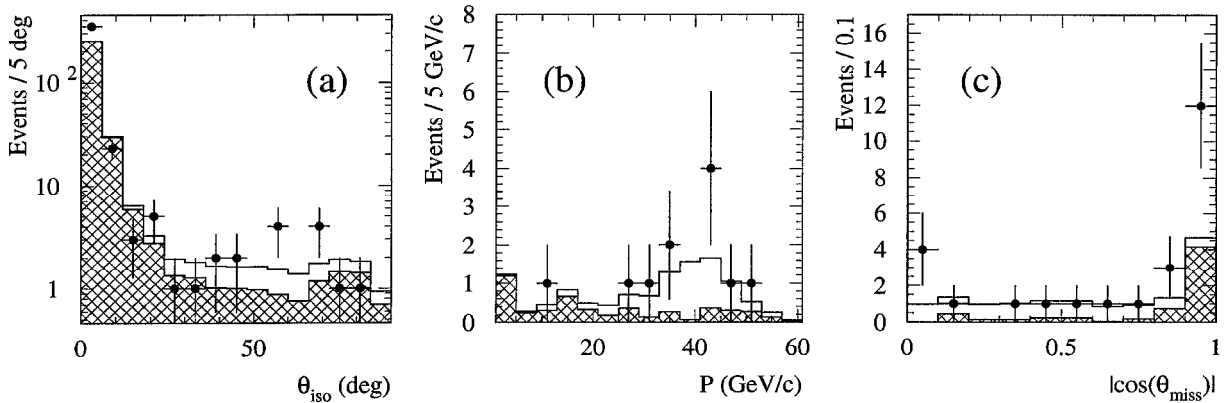
Fig. 2. Semileptonic final state: (a) isolation angle of the lepton; (b) momentum of the lepton; (c) polar angle of the missing momentum. The full lines are the expectations for the fitted signal (white areas) plus the calculated background (cross-hatched areas); data points are shown with statistical error bars. Distribution (a) contains all events with at least 6 charged tracks and a lepton with momentum above 10 GeV/c; for (b) and (c), all selection criteria are applied except the one on the variable described by each plot.
