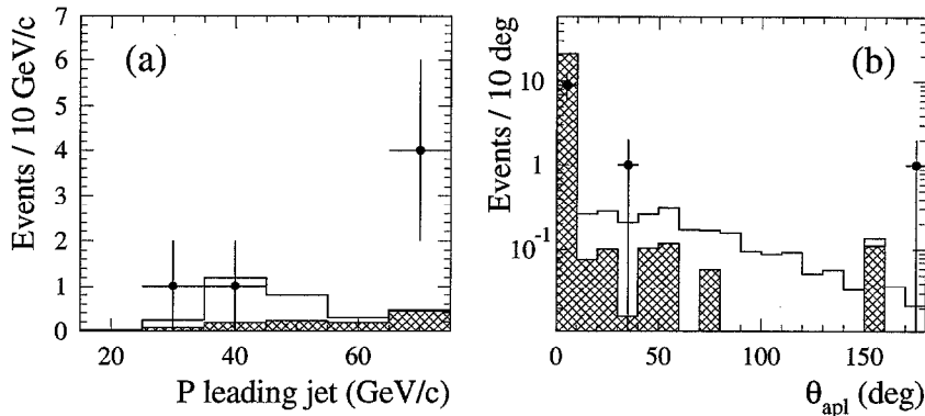
Fig. 3. Fully leptonic final states: (a) momentum of the leading jet; (b) acoplanarity. The full lines are the expectations for the fitted signal (white areas) plus the calculated background (cross-hatched areas), the data points are shown with statistical error bars. All cuts are applied except the one on the variable described by each plot.
