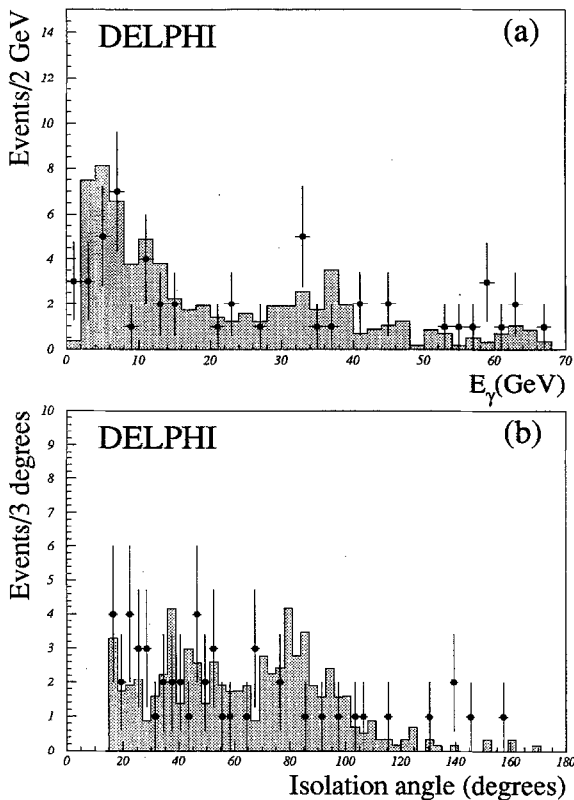
Fig. 2. \ell\ell\gamma\gamma sample: (a) the photon energy and (b) the photon isolation angle. The dots are the data and the shaded area is the simulation.
