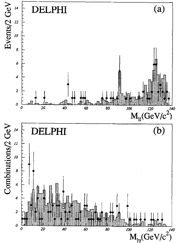
Fig. 1. Invariant mass of lepton pairs (a) and lepton-photon pairs (b) for the l\ell\gamma sample. The dots are the data and the shaded area is the simulation.
