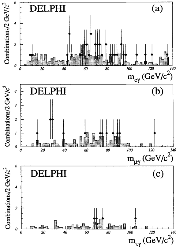
Fig. 3. Invariant masses for all possible lepton-photon combinations in single production searches: electron (a), muon (b) and tau (c) channels. The dots are the data and the shaded area is the simulation.
