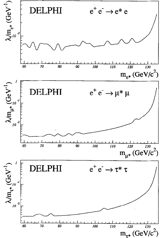
Fig. 4. Single production of excited charged leptons: the line shows the compositeness limits at 95% confidence level of the ratio of the coupling of the excited charged lepton to the mass ( \lambda/m_{\ell^*} ) as a function of the mass for the electron, muon and tau channels.
