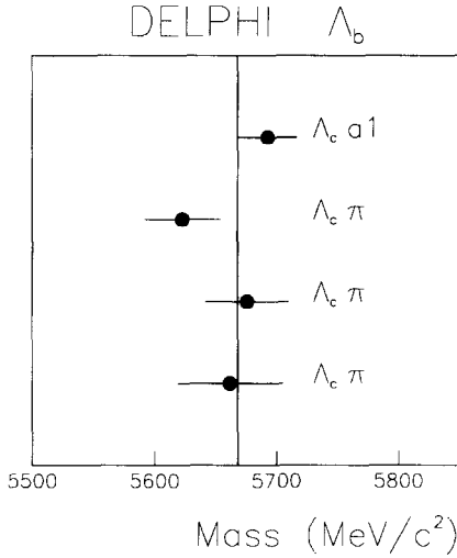
Fig. 3. The masses of the four \Lambda_b^0 candidates in the channels \Lambda_b^0 \rightarrow \Lambda_c^+ \pi^- and \Lambda_b^0 \rightarrow \Lambda_c^+ a_1^- .
