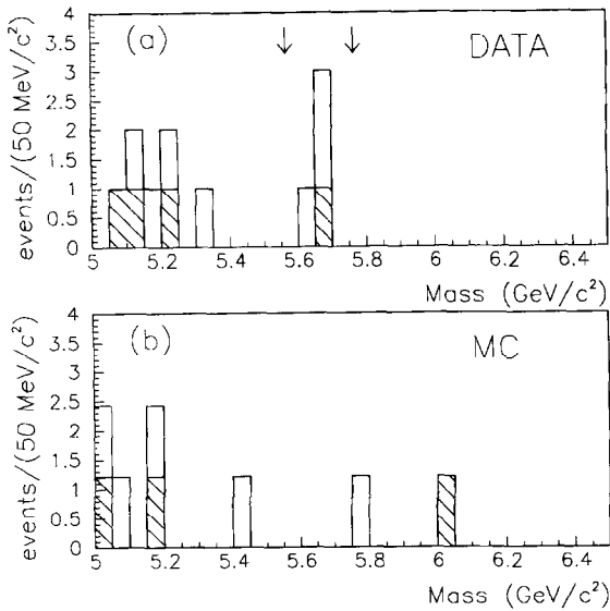
Fig. 1. Invariant mass distributions for the channels \Lambda_b^0 \rightarrow \Lambda_c^+ \pi^- and \Lambda_b^0 \rightarrow \Lambda_c^+ a_1^- for real data (a) and the estimated background distribution from simulation (b). The hatched area corresponds to events in the \Lambda_b^0 \rightarrow \Lambda_c^+ a_1^- channel only. The \Lambda_b^0 mass range is indicated with arrows.
