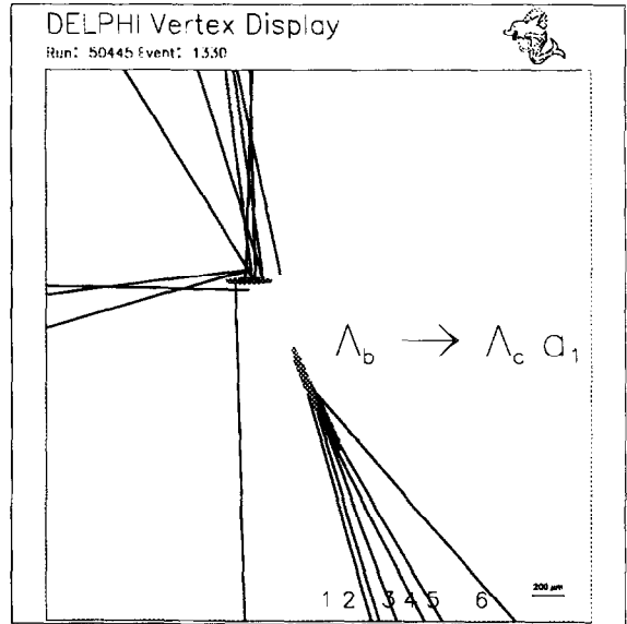
Fig. 2. Display of the vertex region for the \Lambda_b^0 \rightarrow \Lambda_c^+ a_1^- candidate, showing the \Lambda_b^0 and \Lambda_c^+ decay vertices and the primary vertex. The \Lambda_b^0 flies 790 \mu\text{m} . The error ellipses correspond to 1.5 standard deviations. Tracks 1,2 and 6 are the pions from the a_1^- . Tracks 3, 4, and 5 are the kaon, pion, and proton from the \Lambda_c^+ .
