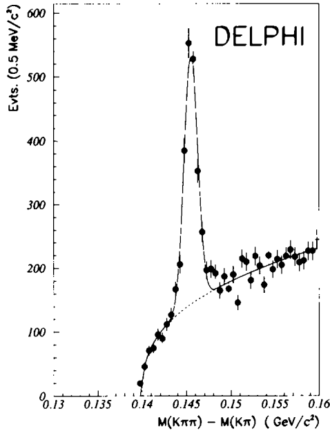
Fig. 1. Distribution of \Delta M = M(K^- \pi^+ \pi^+) - M(K^- \pi^+)
