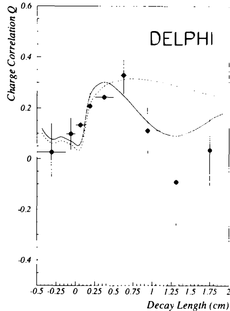
Fig. 3. The charge correlation function Q plotted as a function of the D^0 decay length in cm. The full dots with the error bars represent the data. The full curve is the result of the fit corresponding to \Delta m = 0.50 \hbar/\text{ps} . The dashed curve corresponds to a time independent mixing hypothesis.
