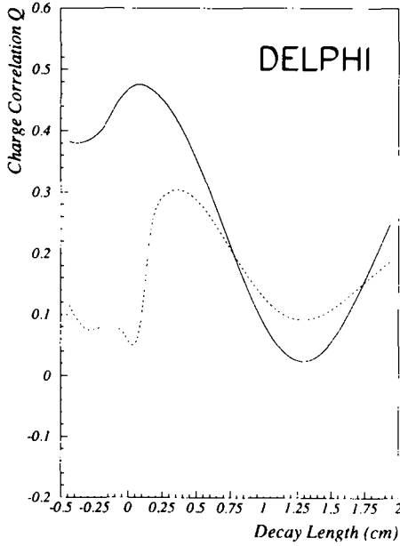
Fig. 2. The charge correlation Q(t) as a function of the D^0 decay length. The full curve corresponds to the expected behaviour for B^0 events generated with \Delta m = 0.50 \text{ h/ps} . The dashed curve includes the contribution from charged B , charm and combinatorial background.
