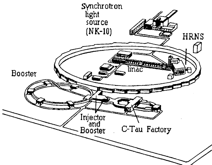
Fig.1. Layout of the JINR storage ring complex.
