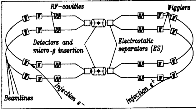
Fig.4. The tau-charm factory storage rings.
