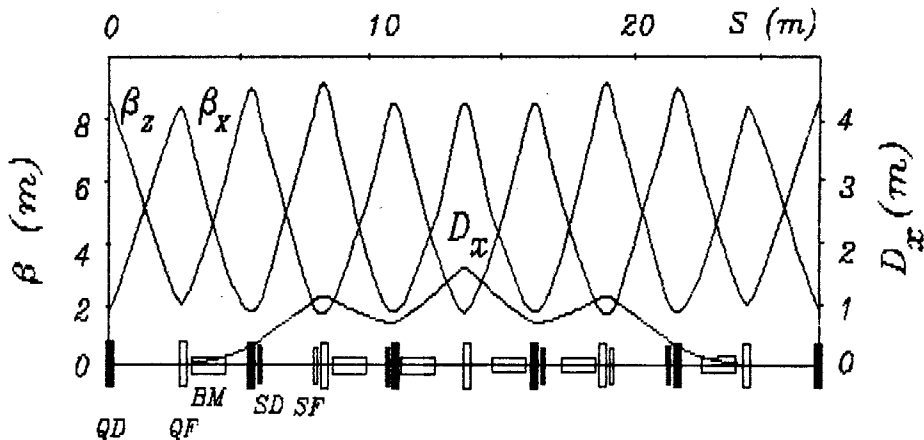
Fig.3. Lattice functions in the booster superperiod.
