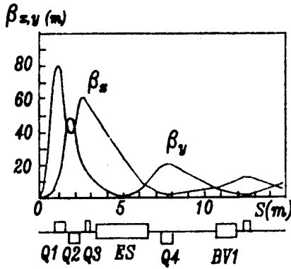
Fig.5. Lattice functions in the interaction region.
